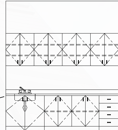
MILLWORK ELEVATION
